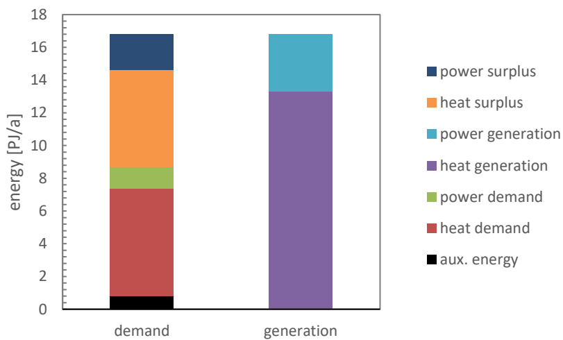
Figure 34 Energy balance case study 4.
