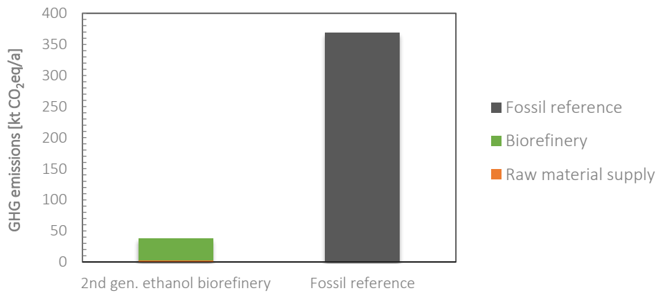
Figure 13 Greenhouse gas emissions of biorefinery compared to reference case study 1.
