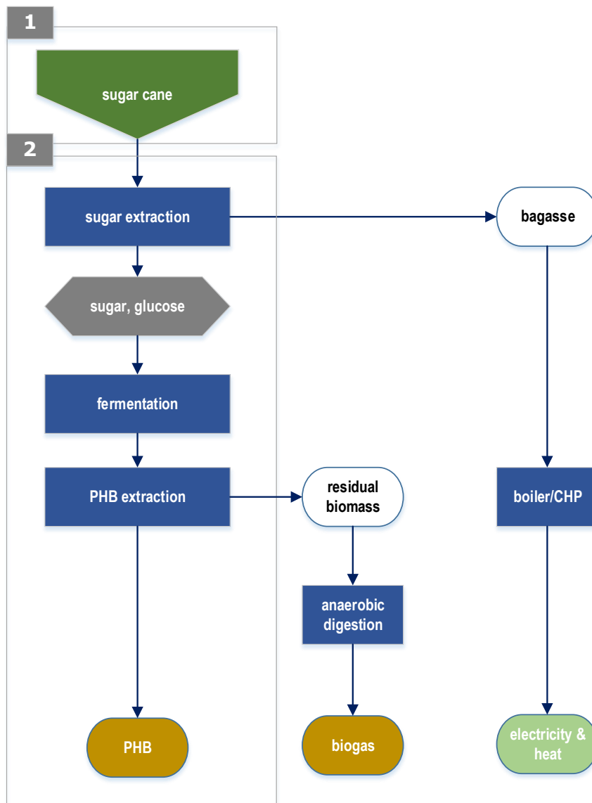
Figure 17 Case study #2: Polyhydroxybutyrate (PHB) biorefinery pathway.
