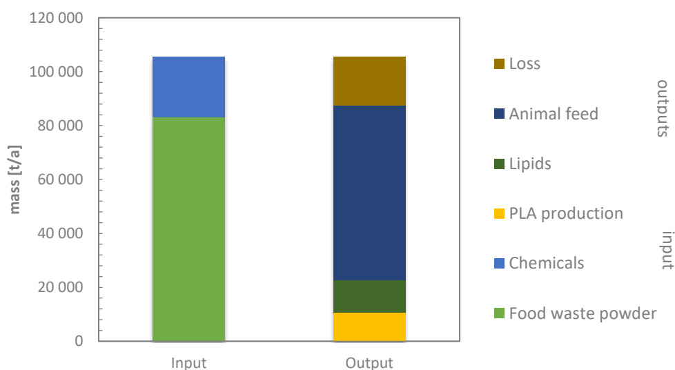
Figure 25 Mass balance case study 3.
