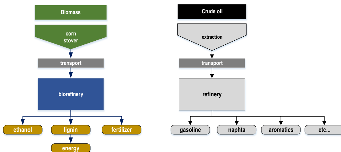
Figure 12 Biorefinery and reference system – value chain case study 1 (cradle-to-gate).
