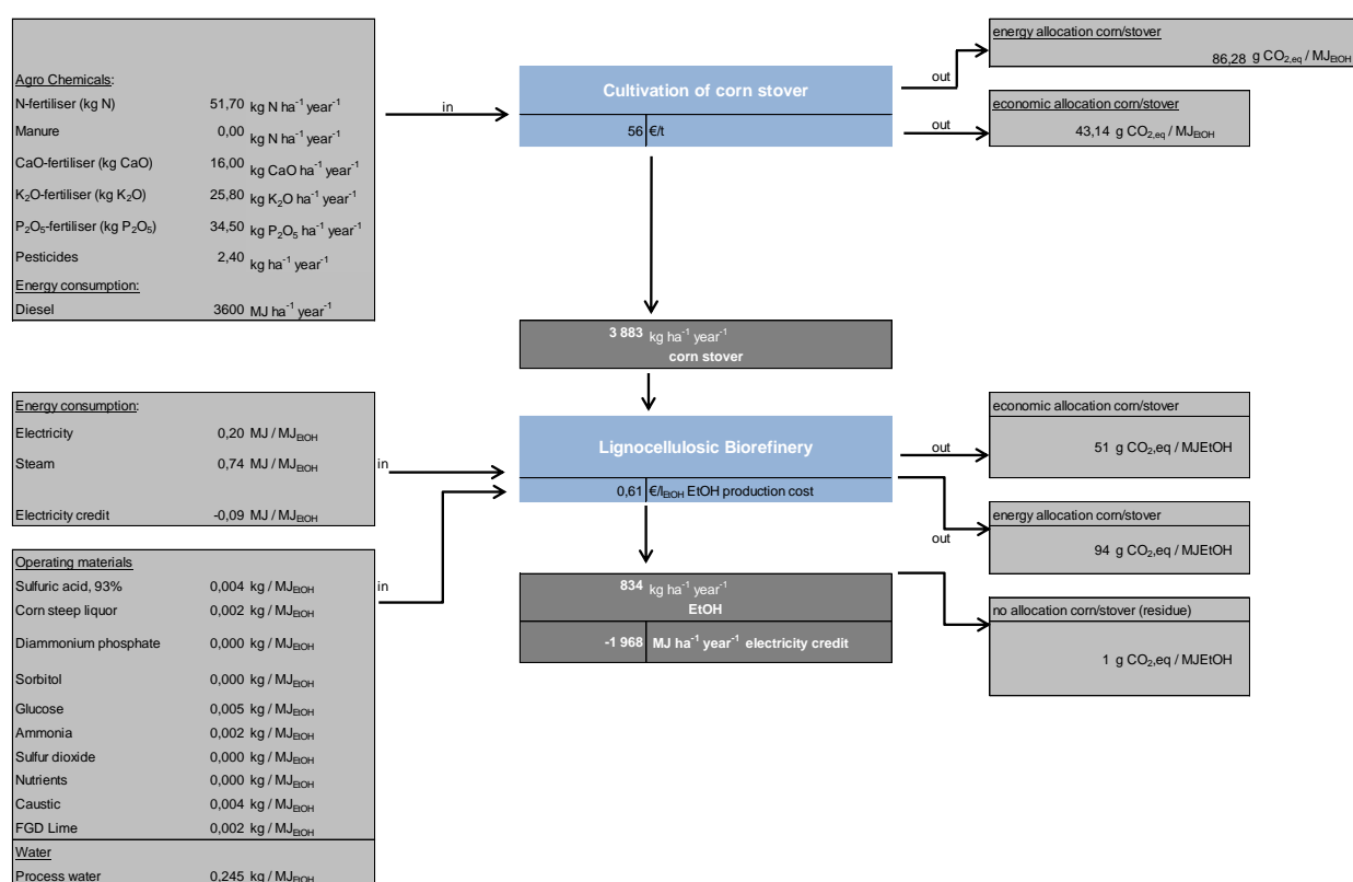
Figure 7 Overview TEE assessment: process pathways bioethanol synthesis from corn stover.
