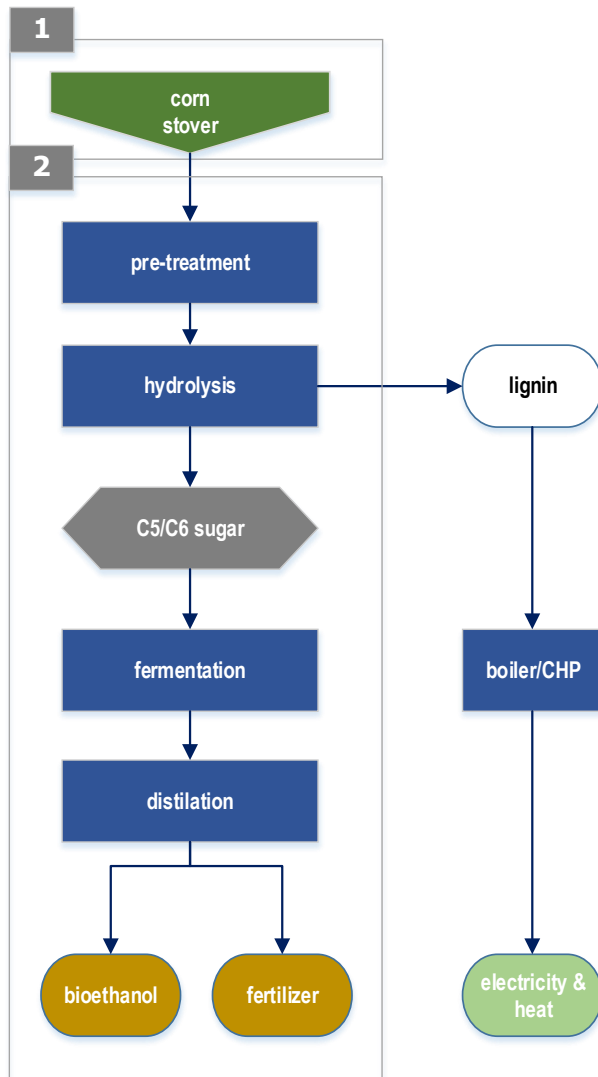
Figure 8 Case study #1: Lignocellulosic bioethanol biorefinery pathway.
