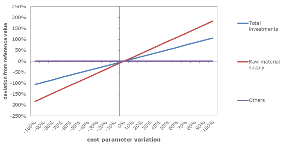
Figure 11 Sensitivity analysis of the cost structure in case study 1.
