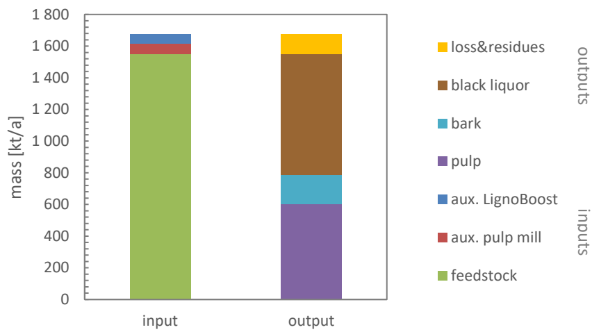
Figure 33 Mass balance case study 4.
