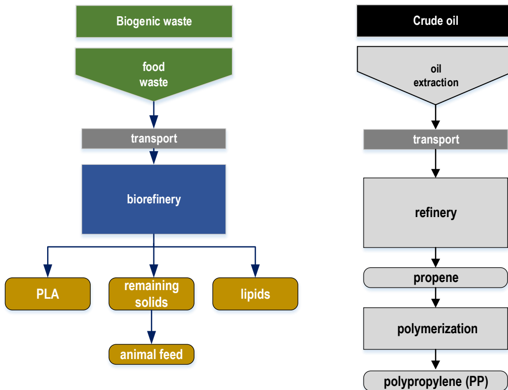
Figure 27 Biorefinery and reference system – value chain case study 3 (cradle to gate).
