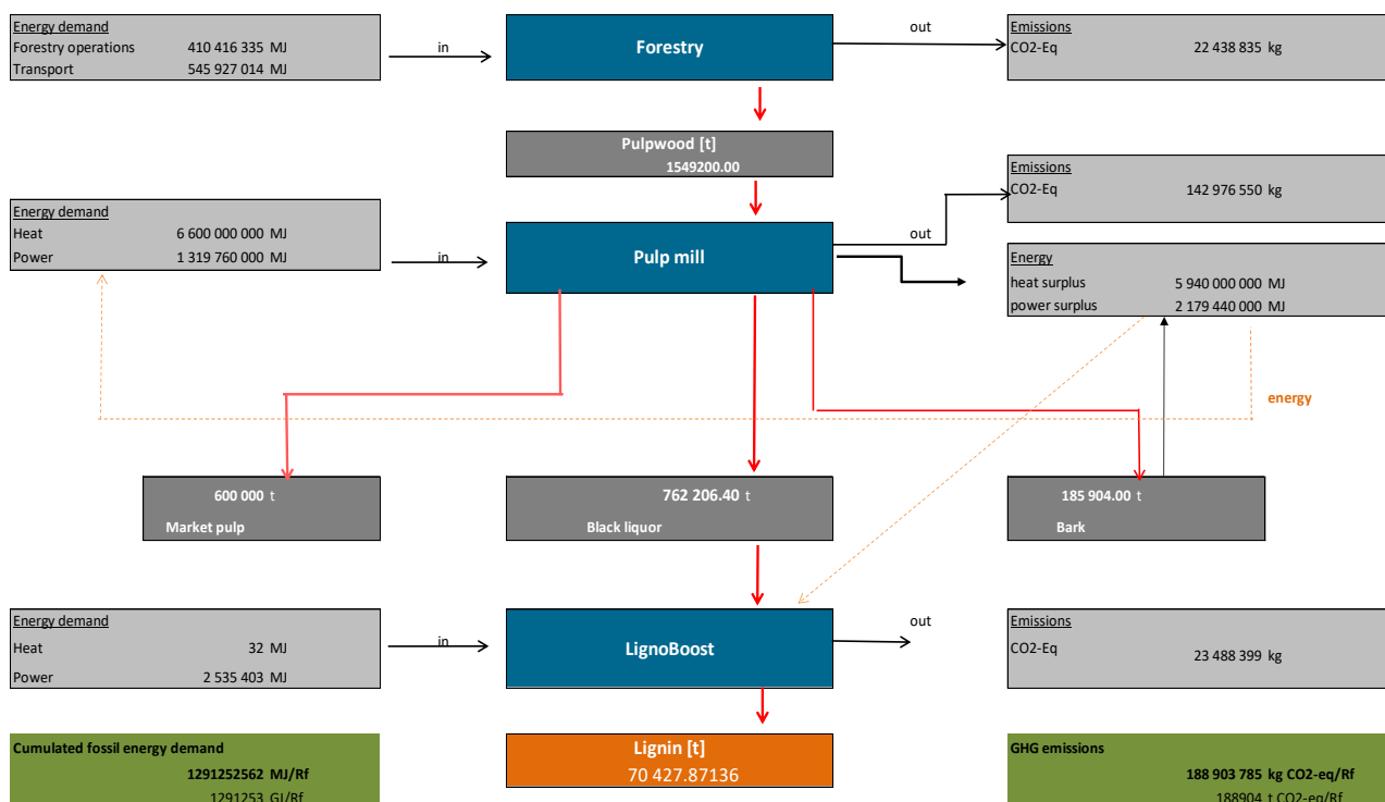
Figure 31 Overview TEE assessment: process pathways lignin from wood chips.
