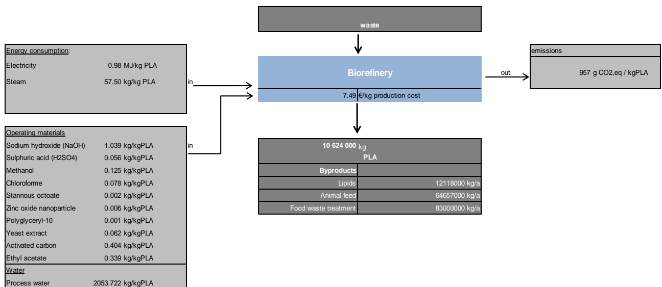
Figure 23 Overview TEE assessment: Process pathway polylactic acid (PLA).
