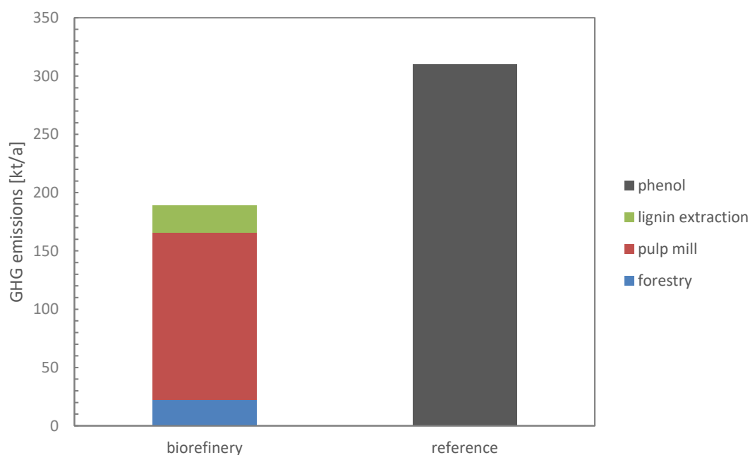
Figure 38 Greenhouse gas emissions of biorefinery compared to reference plant case study 4.
