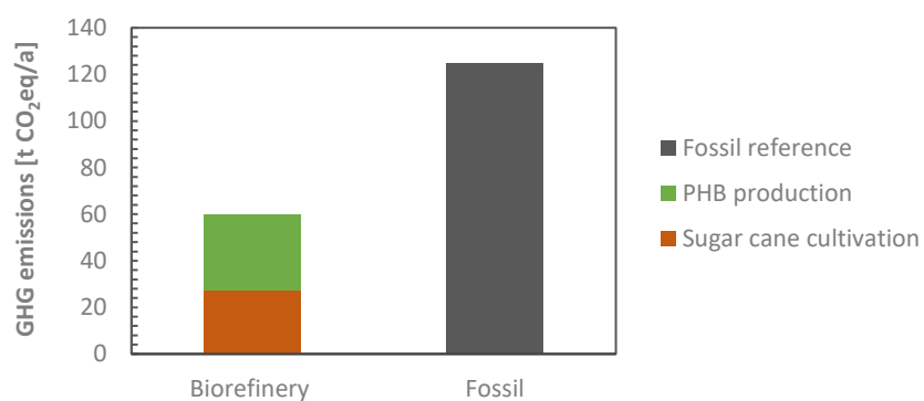
Figure 22 Greenhouse gas emissions of biorefinery compared to reference plant case study 2.
