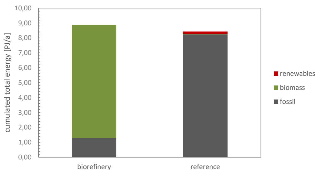
Figure 37 Cumulated energy demand of biorefinery compared to reference plant case study 4.
