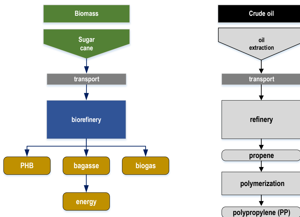
Figure 20 Biorefinery and reference system – value chain case study 2 (cradle to gate)
