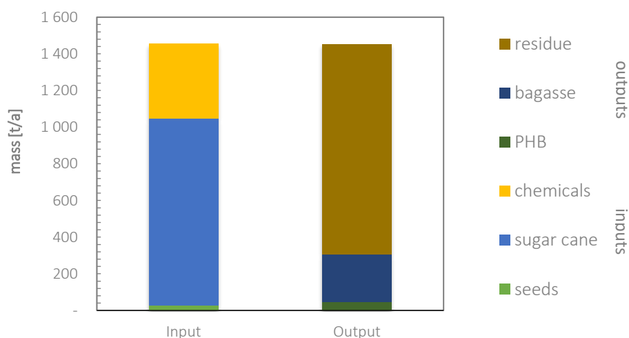
Figure 18 Mass balance case study 2.
