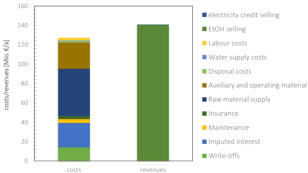
Figure 15 Costs and revenues case study 1.
