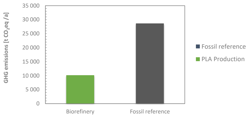
Figure 29 Greenhouse gas emissions of biorefinery compared to reference plant case study 3
