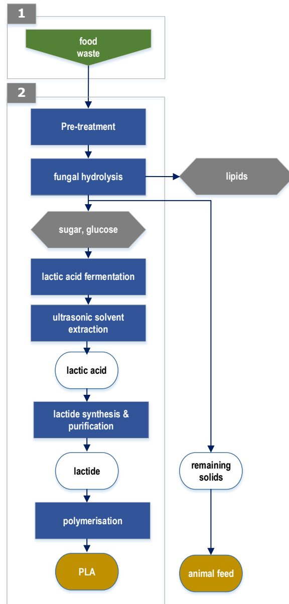
Figure 24 Case study #3: Process pathway PLA from waste.
