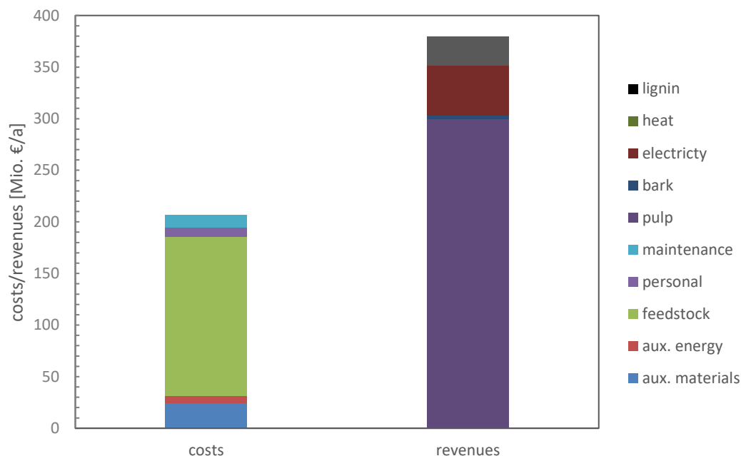
Figure 39 Costs and revenues - case study 4.
