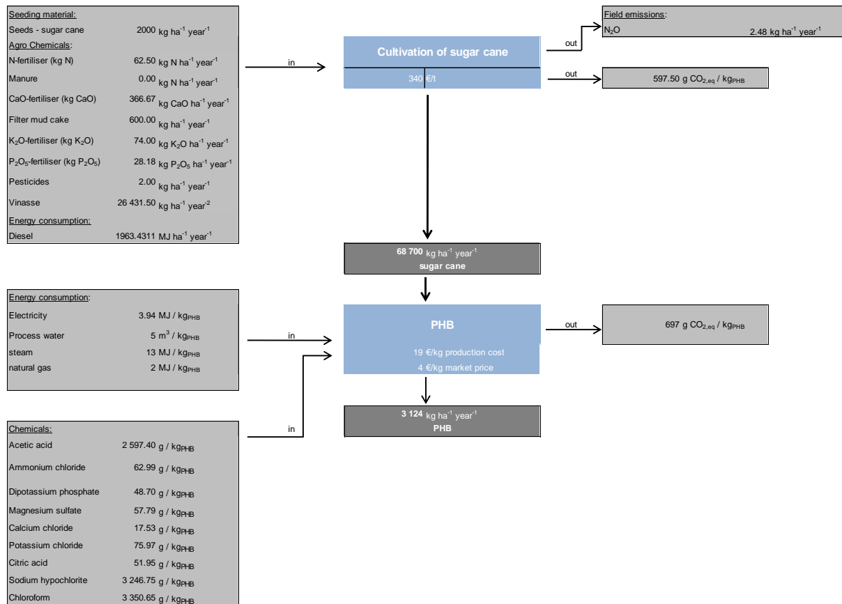
Figure 16 Overview TEE assessment: process pathway PHB from sugar cane.
