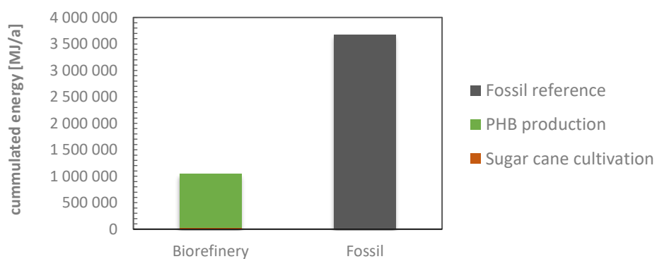
Figure 21 Cumulated energy demand of biorefinery compared to reference plant case study 2.
