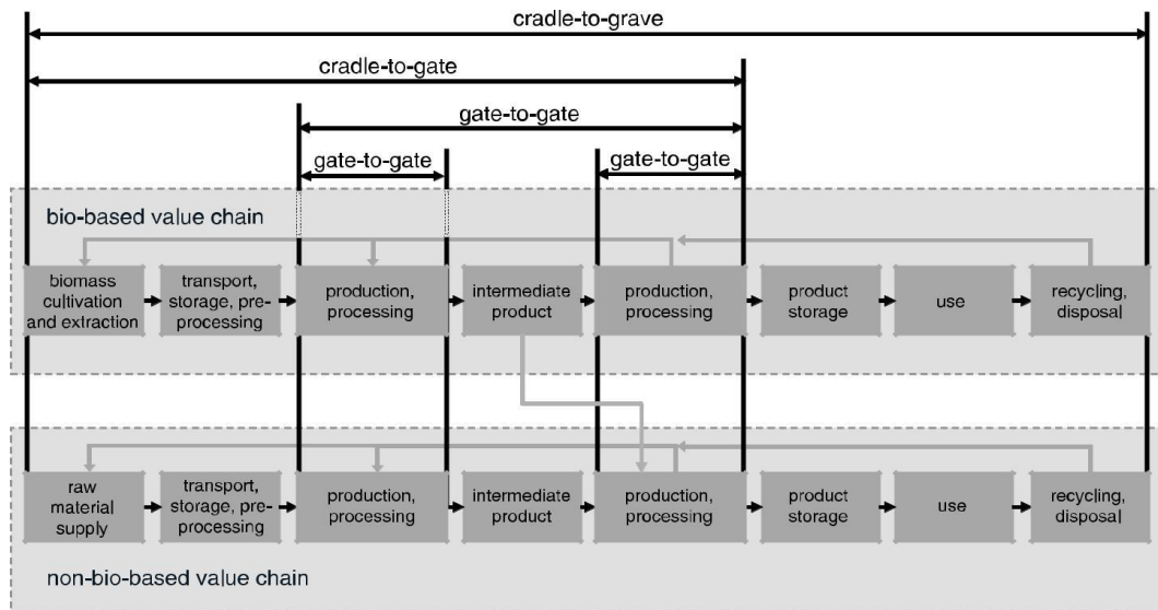
Figure 2 Definitions of system boundaries for biobased and non-biobased value chains (VDI, 2016).
