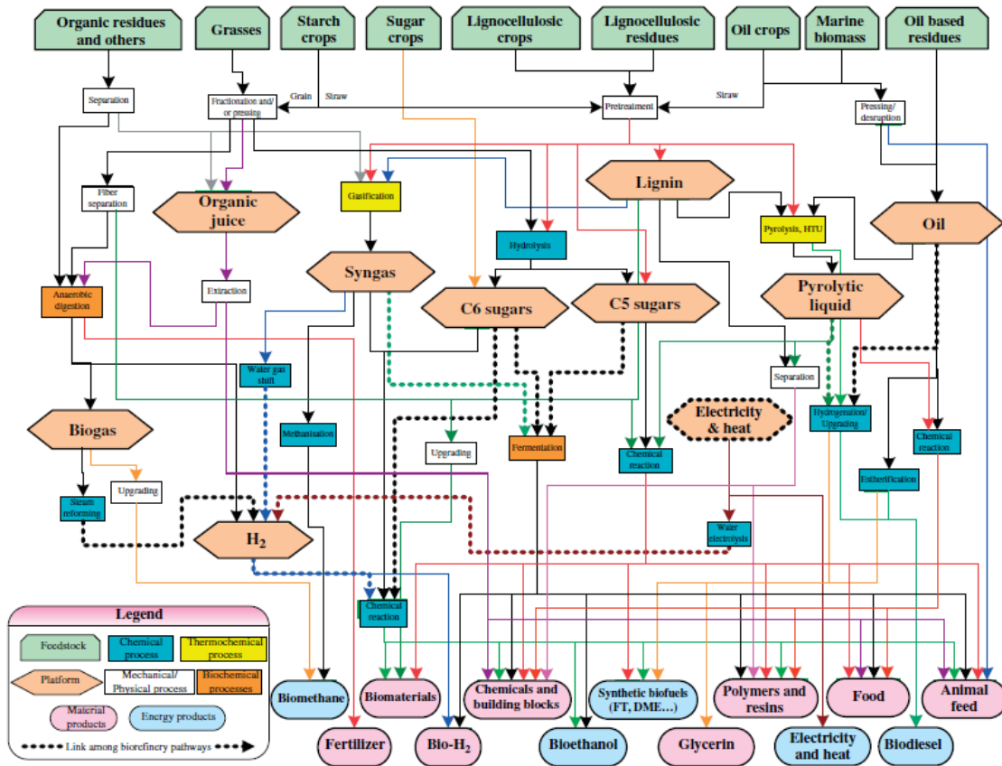
Figure 4 Network where the individual biorefinery systems are combined (Cherubini et al., 2009).
